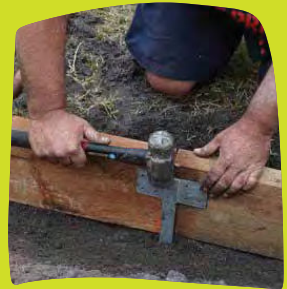
Retaining Stake 16012
